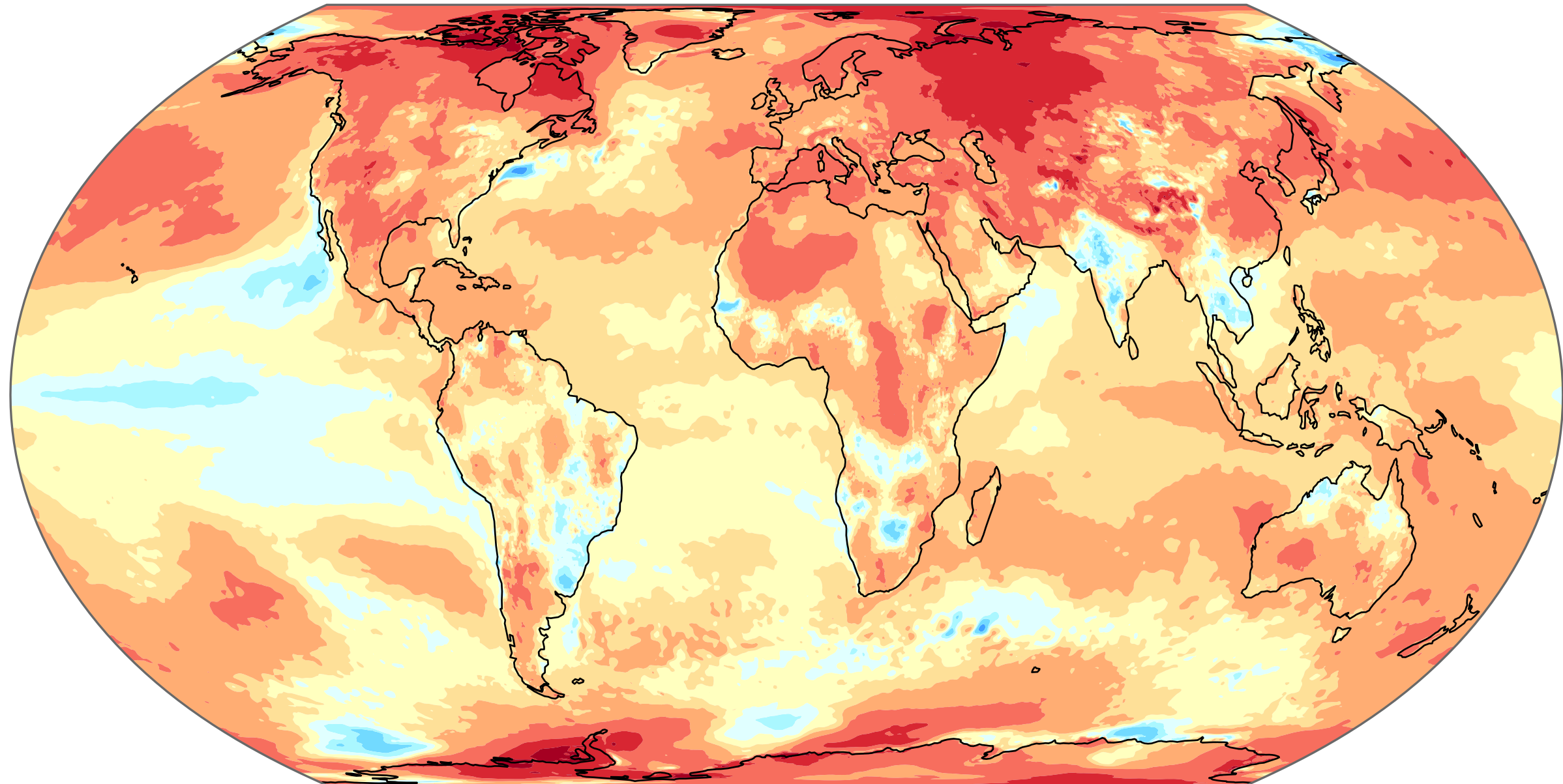
12-month average December 2024 - November 2025 temperature anomaly
