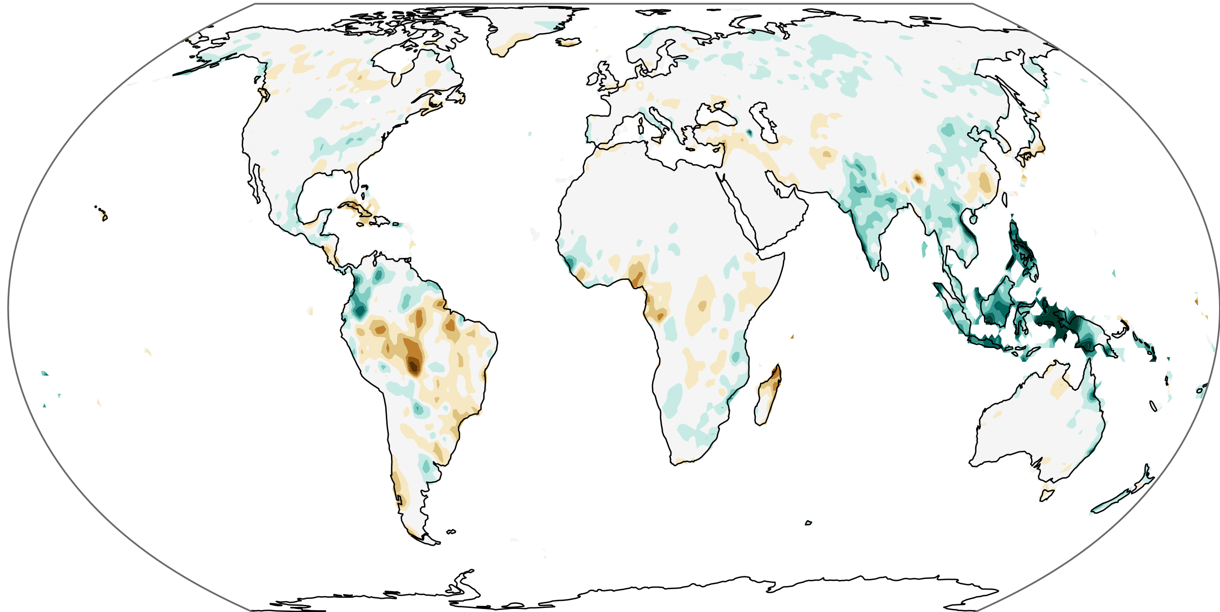
12-month average December 2024 - November 2025 precipitation anomaly
